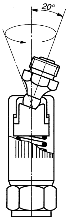
Mod. 450 "SUPERMAXIMA" 4 Jaw fittings 10x1 female
