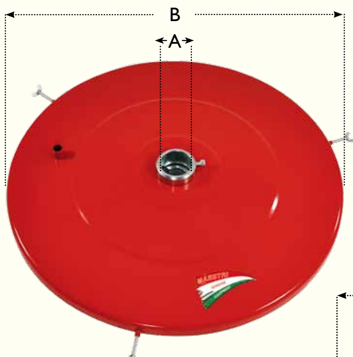
Mod. 366/06 Cover suitable for 20-30kg drums Mod. 367/06 Cover suitable for 50-60kg drums Mod. 368/06 Cover suitable for 200kg drums
